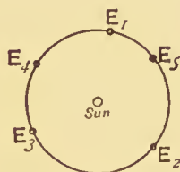
FIG. 12.—True orbits of Earth and Jupiter.
